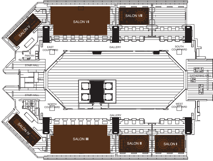
86TH FLOOR
